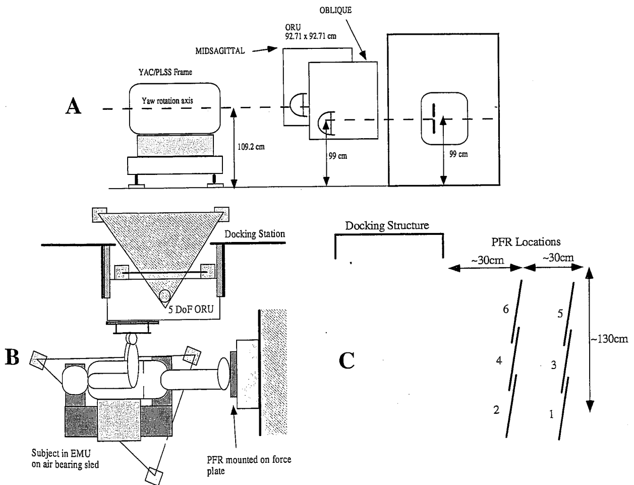
Figure 5. Schematic showing the layout for the PABF test of mass handling.
