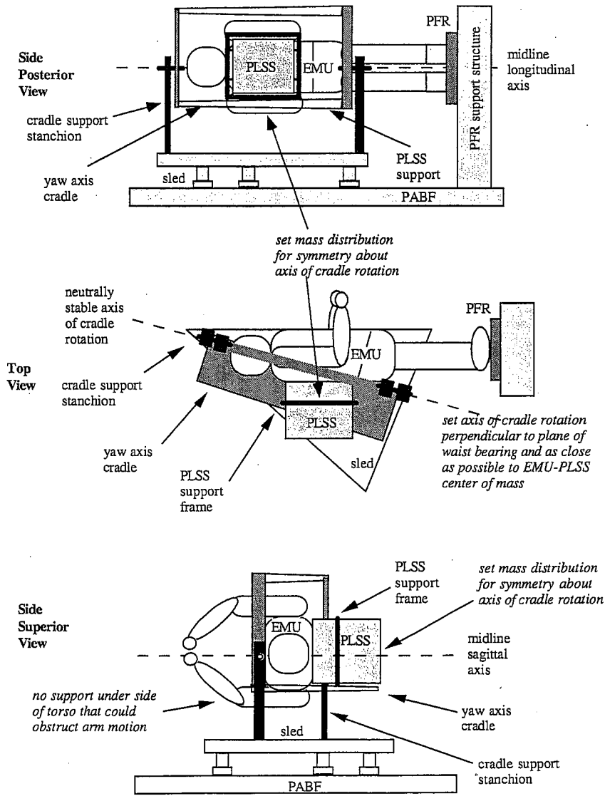
Figure 3. Schematic of YAC-EMU-sled assembly.
