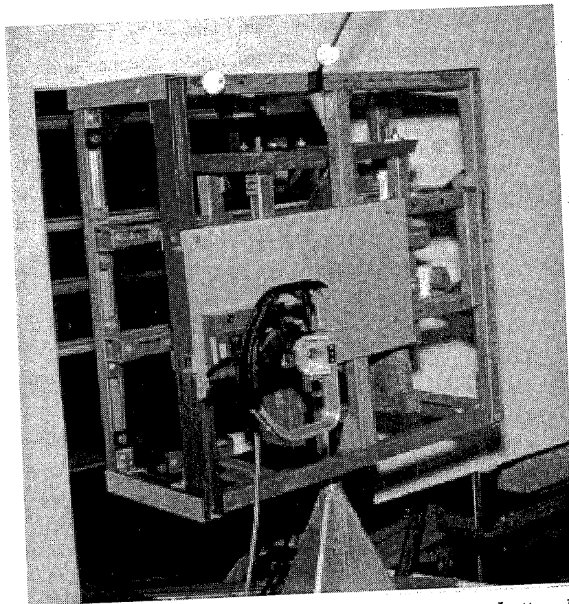
Figure 4. ORU mockup derived from the Rocketdyne battery box.
