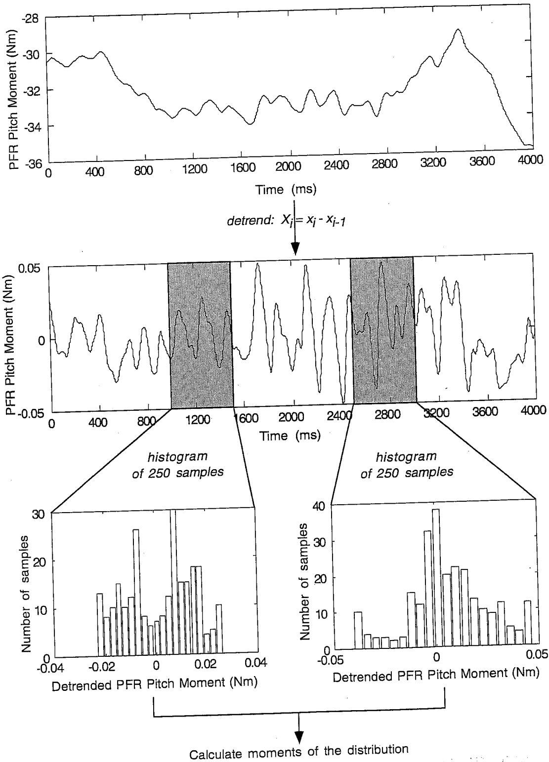
Figure 6. Procedure for deriving update interval distribution moments. Distributions are shown only for two update intervals for clarity. However, distributions are calculated for contiguous update intervals throughout the trial.
